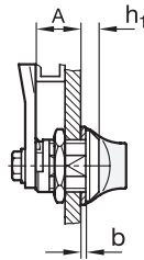
Latches GN 115
