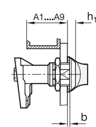
Latches GN 119
