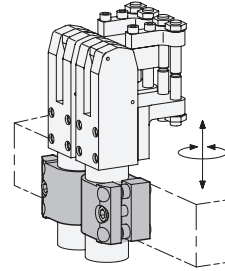
Mounting examples
