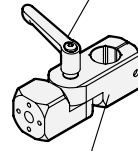
Swivel clamp mounting GN 482, Type P
