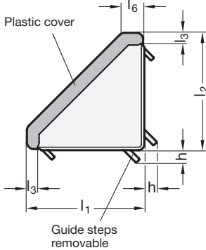
Assembly set for slot width 8 2x T-Nut GN 505 2x Socket head cap screw DIN 7984
