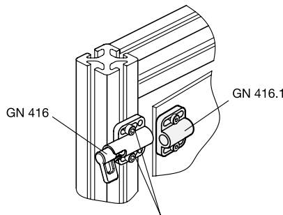
Assembly set GN 965 / GN 968
