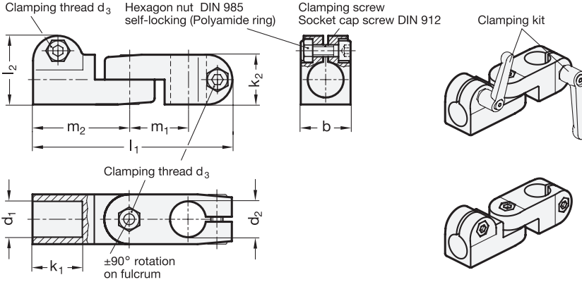
3 Identification No. 2 with 3 Stainless Steel-Clamping screws DIN 912
