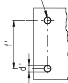
Drilling template Holes without burrs and chamfer
