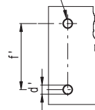
Drilling template Holes without burrs and chamfer
