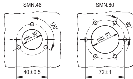
Drilling templates
