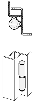
Example of installation
