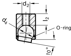
Application example of different clamping pads with O-ring
