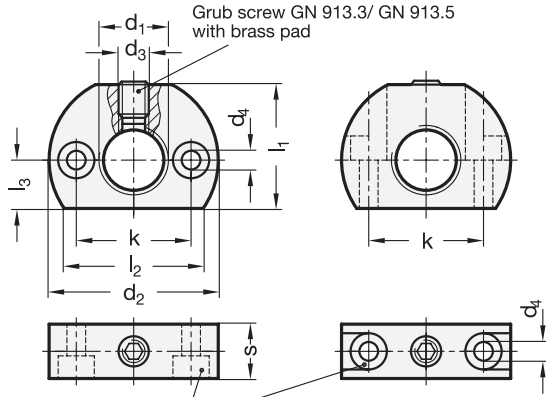
Counterbored for cap screws DIN 912- M4/5
