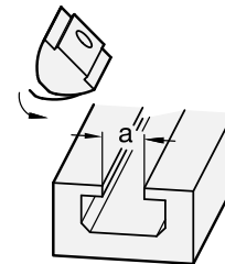
T-nuts to swivel in
