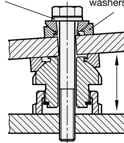
Spherical levelling washers GN 350.3
