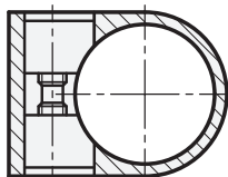
Shaft clamping unit
