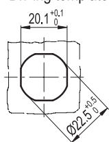
Drilling template
