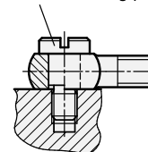
Cylinder head shoulder bolt GN 732 used as bearing pin
