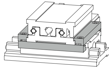
Assembly example
