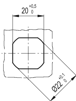
Drilling template
